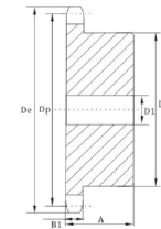
TYPE B
