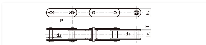
钢制套筒链 STEEL BUSH CHAINS
