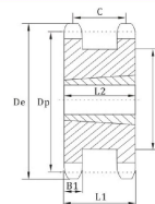
TYPE B BUSH TYPE A
