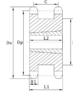
TYPER BUSH TYPE A
