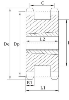
TYPER BUSH TYPE A
