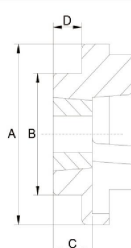
H型联轴器外形尺寸 (锥孔) H Flange (Taper Bored)
