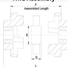
HRC联轴器 HRC Assembly
