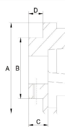
B型联轴器外形尺寸 (锥孔) B Flange (Pilot Bore)
