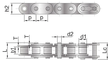
A 系列短节距直板精密滚子链 Short pitch precision roller chain with straight plate (A series)
