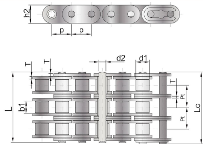
A 系列短节距直板精密滚子链 Short pitch precision roller chain with straight plate (A series)
