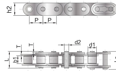
B 系列短节距直板精密滚子链 Short pitch precision roller chain with straight plate (B series)
