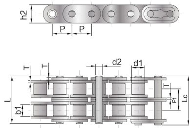
B 系列短节距直板精密滚子链 Short pitch precision roller chain with straight plate (B series)
