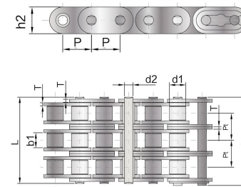
B 系列短节距直板精密滚子链 Short pitch precision roller chain with straight plate (B series)
