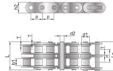
A 系列短节距直板精密滚子链 Short pitch precision roller chain with straight plate (A series)
