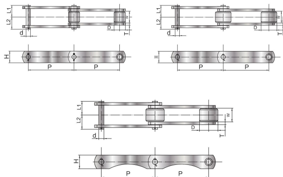
套筒滚子输送链 Conveyor roller chain
