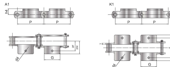
带附件套筒输送链 Conveyor bushing chain with attachment
