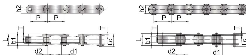
双节距输送链 Double pitch conveyor chain
