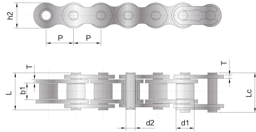
其它单排滚子链 Other single roller chain
