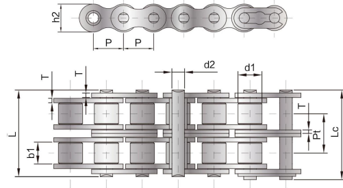
A 系列短节距双排精密滚子链 Short pitch precision duplex roller chain (A series)
