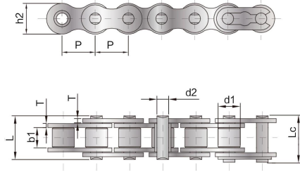
B 系列短节距单排精密滚子链 Short pitch precision single roller chain (B series)
