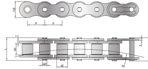
侧弯链 Side bow chain
