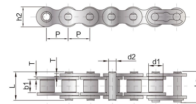
A 系列短节距单排精密滚子链 Short pitch precision single roller chain (A series)
