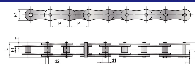
双节距传动链 Double pitch driving chain
