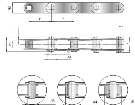
FV 系列输送链 Conveyor chain (FV Series)
