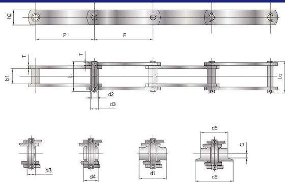
FV 系列输送链 Conveyor chain (FV Series)
