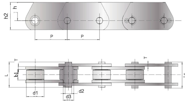
FVT 系列输送链 Conveyor chain (FVT Series)
