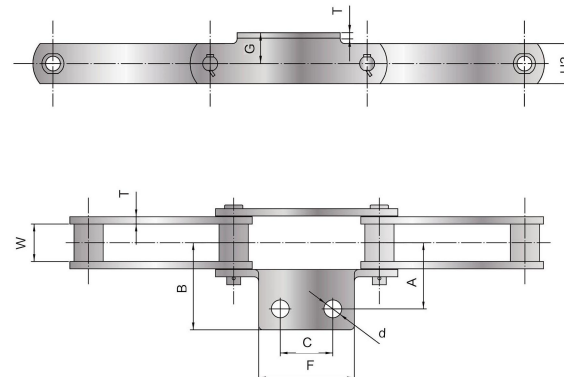
HSC 不锈钢链附件 A2 HSC stainless steel chain with attachment A2
