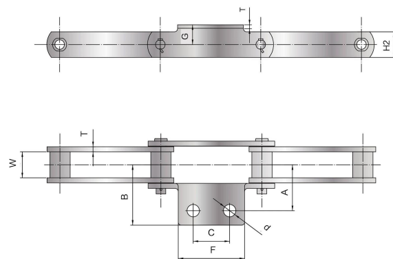
HSS 不锈钢链附件 A2 HSS stainless steel chain with attachment A2
