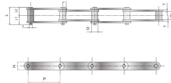
HSC 不锈钢链 HSC stainless steel chain
