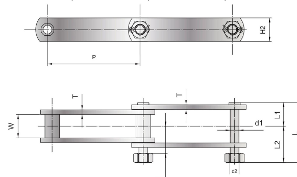
HSC 不锈钢链附件 D22 HSC stainless steel chain with attachment D22
