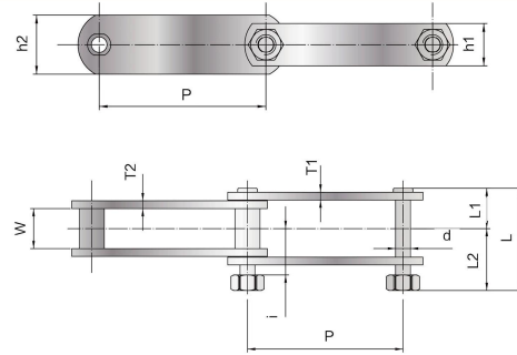
HSS 不锈钢链 HSS stainless steel chain
