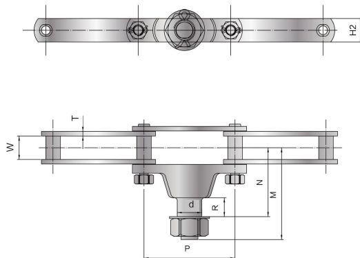
HSC 不锈钢链附件 T1 HSC stainless steel chain with attachment T1
