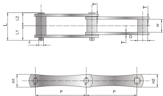
SAV 不锈钢链 SAV stainless steel chain
