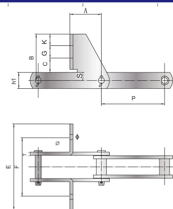
HSS 不锈钢链附件 SF4 HSS stainless steel chain with attachment SF4
