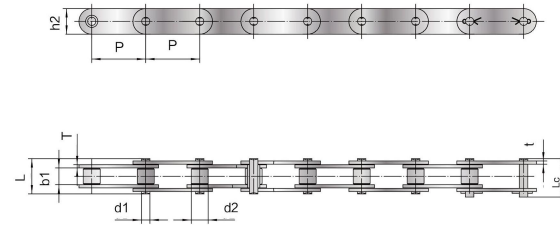
木材输送链 Lumber conveyor chain
