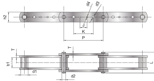
木材输送链 (3939 系列) Lumber conveyor chain (3939 series)
