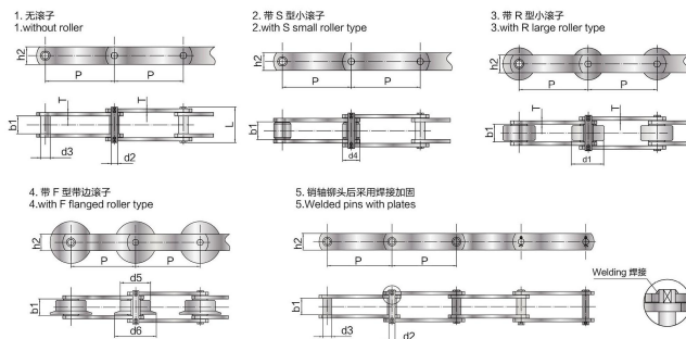
M 系列输送链 Conveyor chain (M series)
