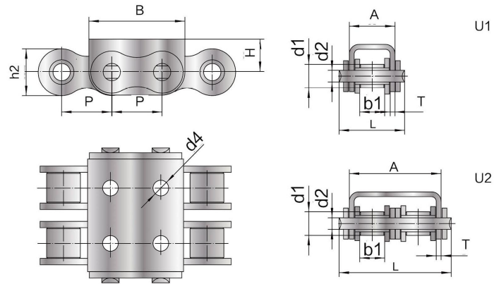
U 型附件滚子链 Roller chain with U type attachment
