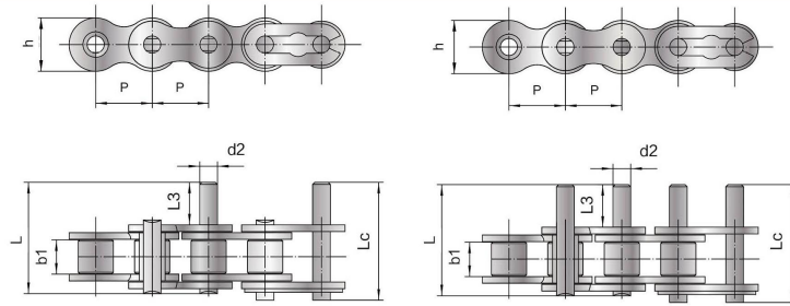
短节距带加长销输送链 Short pitch conveyor chain with extended pin
