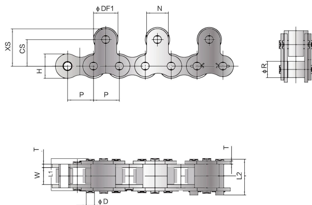
单排顶置滚轮链 Single strand top roller conveyor chain
