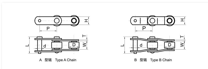
糖机链 CHAINS FOR SUGAR PLANT
