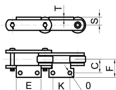
A2附件 A2 Attachment
