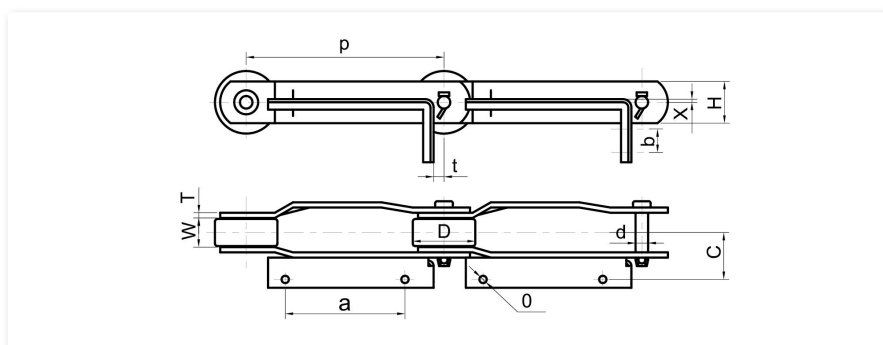
复烤机烟机链条 CHAINS FOR TABACOO BAKING MACHINE
