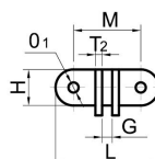
C型飞翼尺寸 Dimension Diagram of Flight Wing Attachment(C Type)
